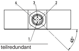
M12 Pinbelegung M12 pin assignment
