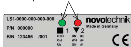
Beispiel LS1 Typenschild. Example of LS1 type label.
